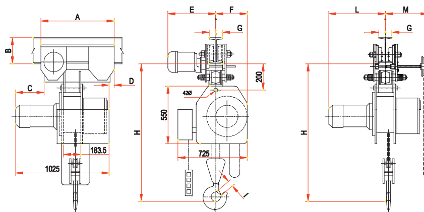
Electric chain hoist with electric trolley
